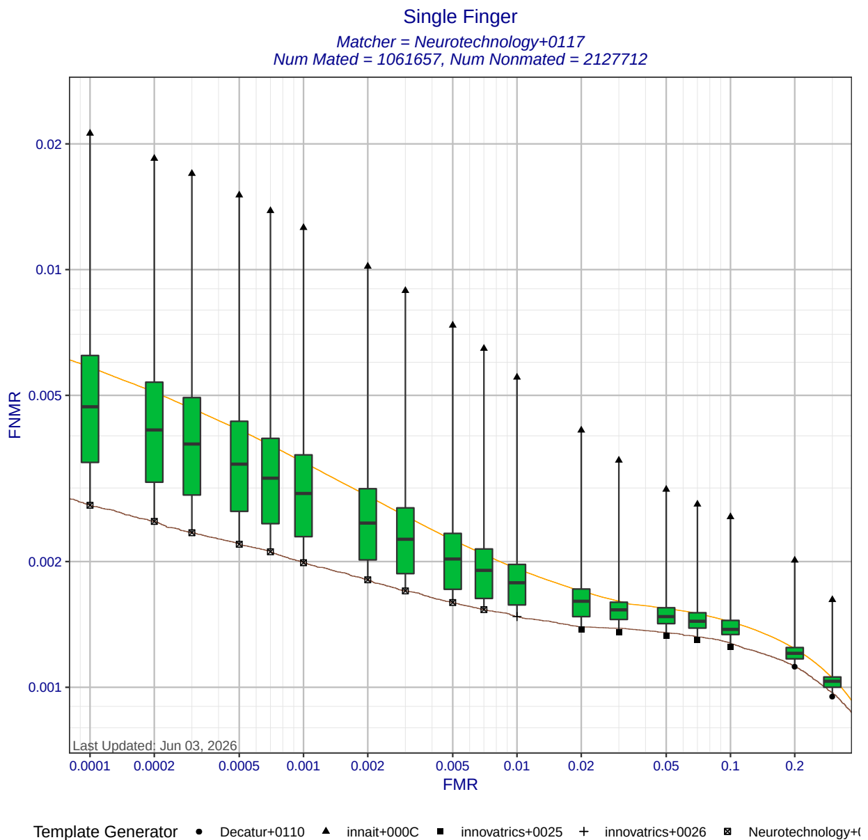
Figure 2: Single finger DET statistics for matcher Neurotechnology+0117. Each box shows the distribution of FNMRs at a fixed FMR across all MINEX III compliant template generators. The ends of the whiskers show the minimum and maximum FNMRs. The orange DET curve shows pooled performance against all template generators.
