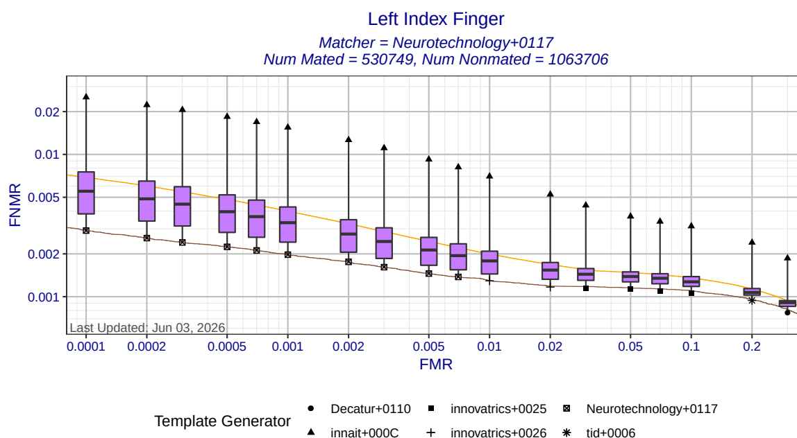
Figure 4: Left index finger DET statistics for matcher Neurotechnology+0117. Each box shows the distribution of FNMRs at a fixed FMR across all MINEX III compliant template generators. The ends of whiskers show the minimum and maximum FNMRs. The orange DET curve shows pooled performance against all template generators.
