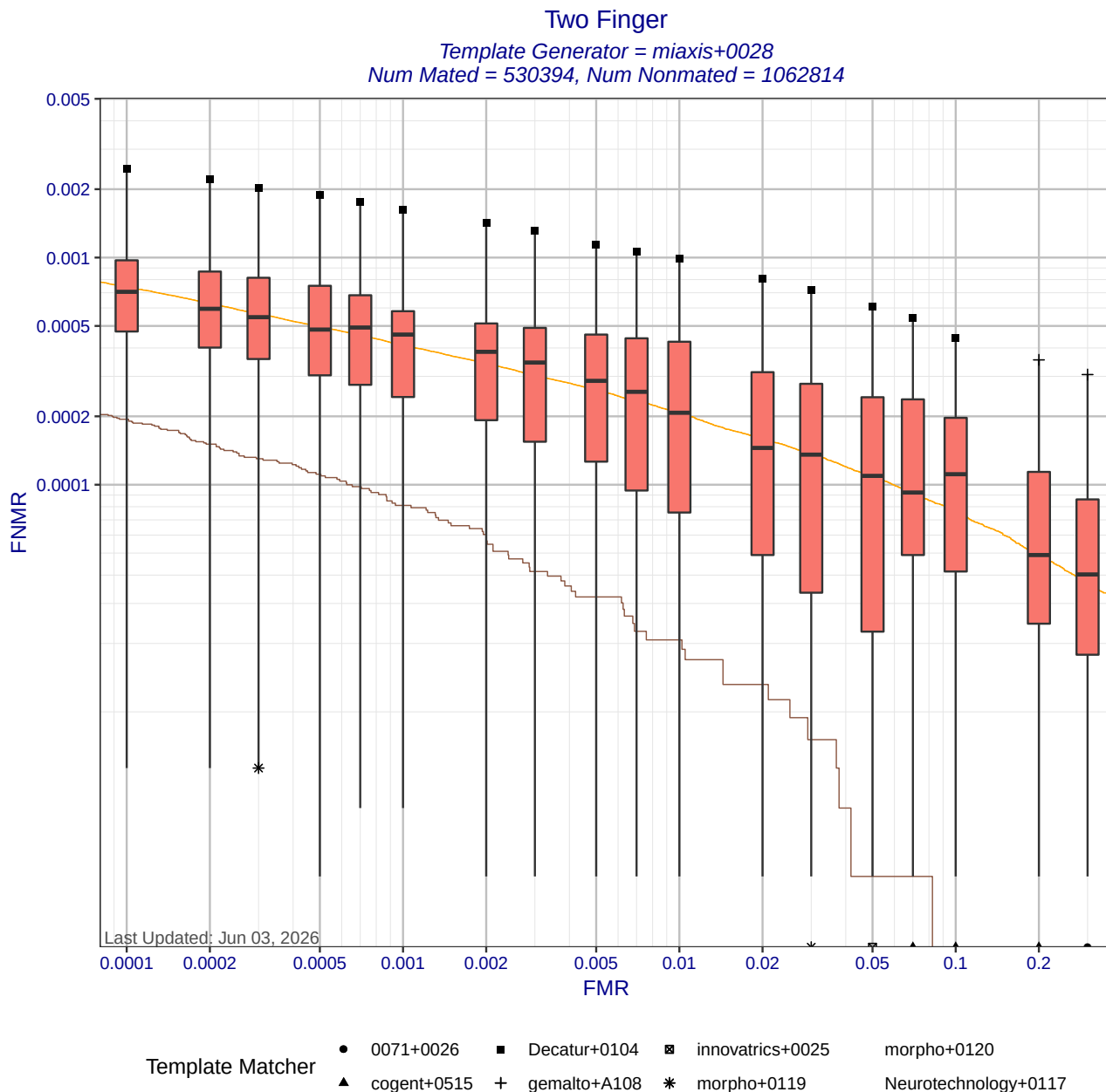
Figure 6: Two Finger DET statistics for template generator miaxis+0028. Each box shows the distribution of FNMRs at a fixed FMR across different matchers. The whisker ends show the minimum and maximum FNMRs. The brown curve shows the DET curve when the matcher and template generators were submitted by the same participant. The orange DET curve shows pooled performance when all matchers use templates created by miaxis+0028. Score-level fusion is achieved by averaging the scores for left and right index fingers.
