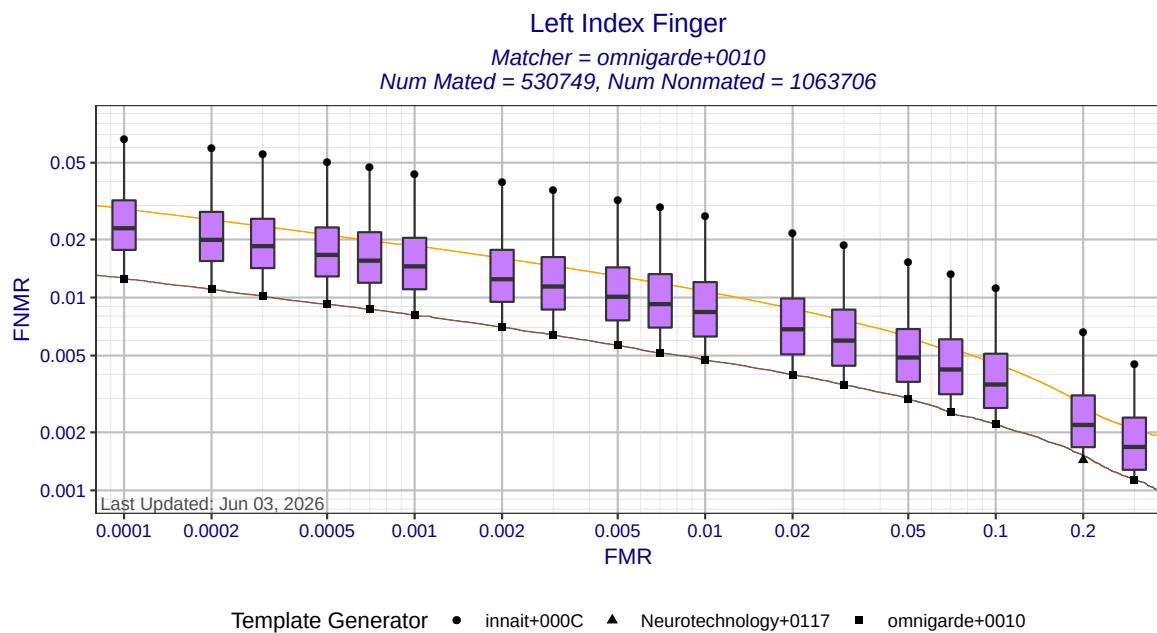
Figure 4: Left index finger DET statistics for matcher omnigarde+0010. Each box shows the distribution of FNRs at a fixed FMR across all MINEX III compliant template generators. The ends of whiskers show the minimum and maximum FNRs. The orange DET curve shows pooled performance against all template generators.
