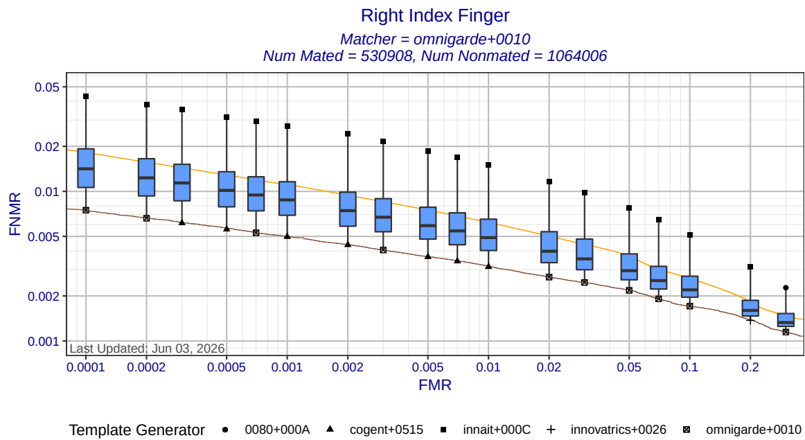
Figure 3: Right index finger DET statistics for matcher omnigarde+0010. Each box shows the distribution of FNR at a fixed FMR across all MINEX III compliant template generators. The ends of the whiskers show the minimum and maximum FNRs. The orange DET curve shows pooled performance against all template generators.
