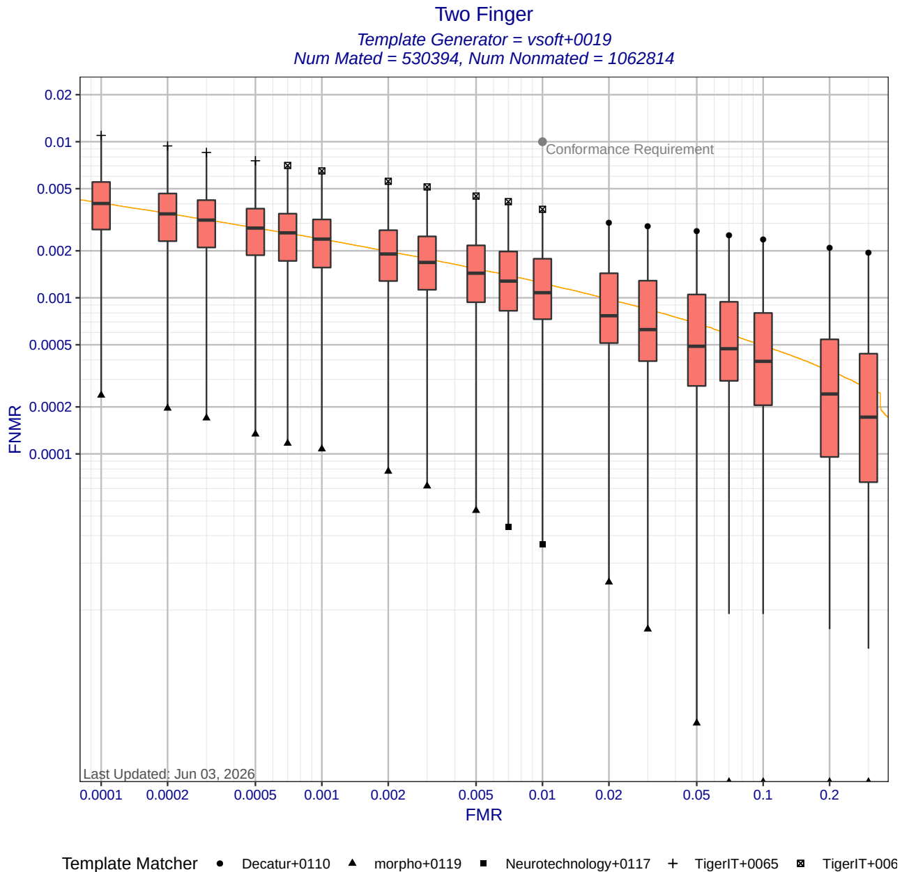
Figure 6: Two Finger DET statistics for template generator vsoft+0019. Each box shows the distribution of FNMrs at a fixed FMR across different matchers. The whisker ends show the minimum and maximum FNMrs. The orange DET curve shows pooled performance when all matchers use templates created by vsoft+0019. Score-level fusion is achieved by averaging the scores for left and right index fingers.
