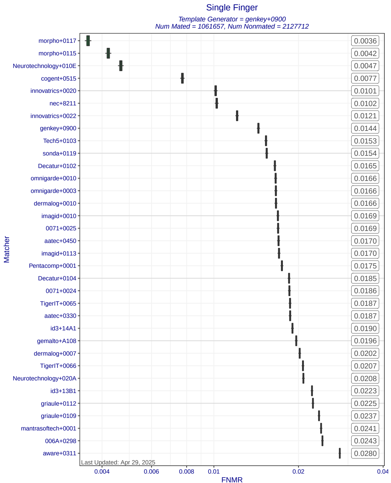
Figure 5: Single Finger FNMRs at FMR=0.0001 when MINEX III compliant matchers compare templates created by template generator genkey+0900. Each box represents uncertainty about the true FNMR. The box edges mark the 50% confidence intervals while the whiskers mark the 90% confidence intervals. The numbers on the right show the actual computed FNMRs.
