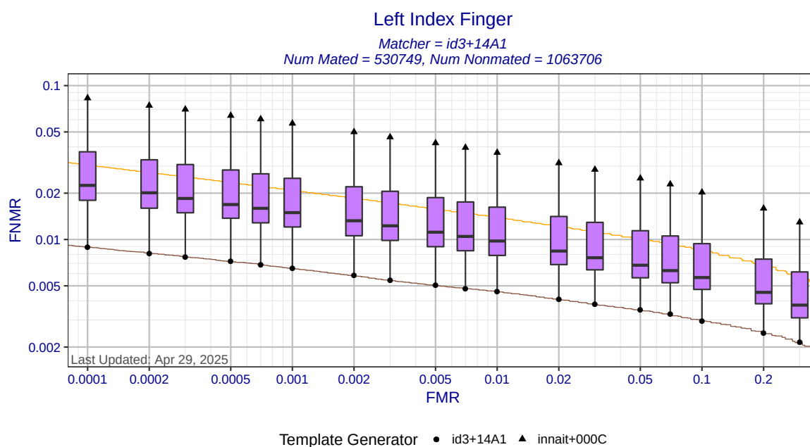
Figure 4: Left index finger DET statistics for matcher id3+14A1. Each box shows the distribution of FNRs at a fixed FMR across all MINEX III compliant template generators. The ends of whiskers show the minimum and maximum FNRs. The orange DET curve shows pooled performance against all template generators.
