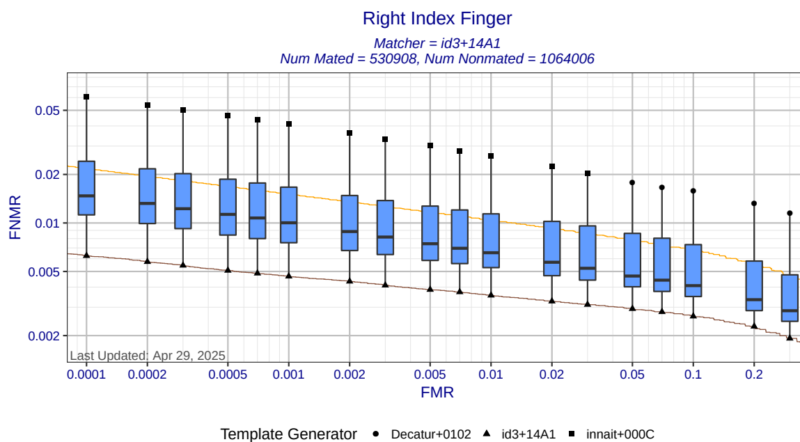
Figure 3: Right index finger DET statistics for matcher id3+14A1. Each box shows the distribution of FNR at a fixed FMR across all MINEX III compliant template generators. The ends of the whiskers show the minimum and maximum FNRs. The orange DET curve shows pooled performance against all template generators.
