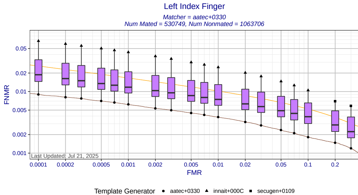
Figure 4: Left index finger DET statistics for matcher aatec+0330. Each box shows the distribution of FNMRs at a fixed FMR across all MINEX III compliant template generators. The ends of the whiskers show the minimum and maximum FNMRs. The orange DET curve shows pooled performance against all template generators.
