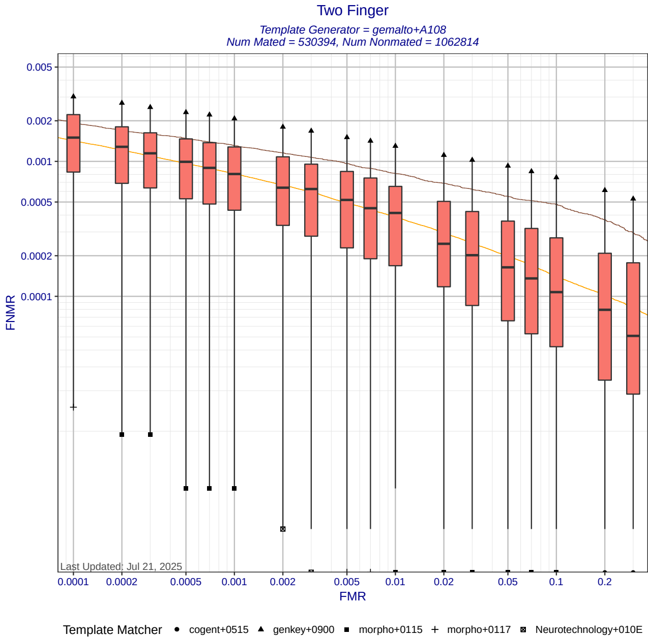
Figure 6: Two Finger DET statistics for template generator gemalto+A108. Each box shows the distribution of FNMIRs at a fixed FMR across different matchers. The whisker ends show the minimum and maximum FNMIRs. The brown curve shows the DET curve when the matcher and template generators were submitted by the same participant. The orange DET curve shows pooled performance when all matchers use templates created by gemalto+A108. Score-level fusion is achieved by averaging the scores for left and right index fingers.
