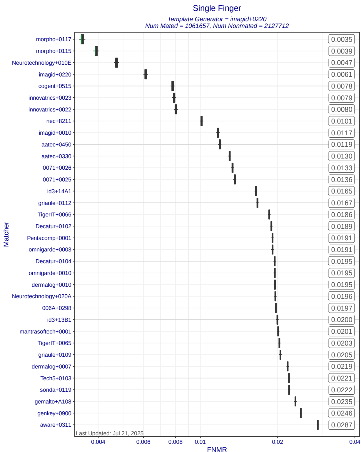
Figure 5: Single Finger FNMRs at FMR=0.0001 when MINEX III compliant matchers compare templates created by template generator imagid+0220. Each box represents uncertainty about the true FNMR. The box edges mark the 50% confidence intervals while the whiskers mark the 90% confidence intervals. The numbers on the right show the actual computed FNMRs.
