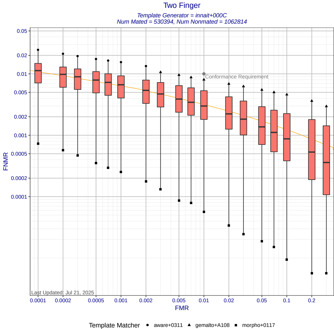
Figure 6: Two Finger DET statistics for template generator innait+000C. Each box shows the distribution of FNMNRs at a fixed FMR across different matchers. The whisker ends show the minimum and maximum FNMNRs. The orange DET curve shows pooled performance when all matchers use templates created by innait+000C. Score-level fusion is achieved by averaging the scores for left and right index fingers.
