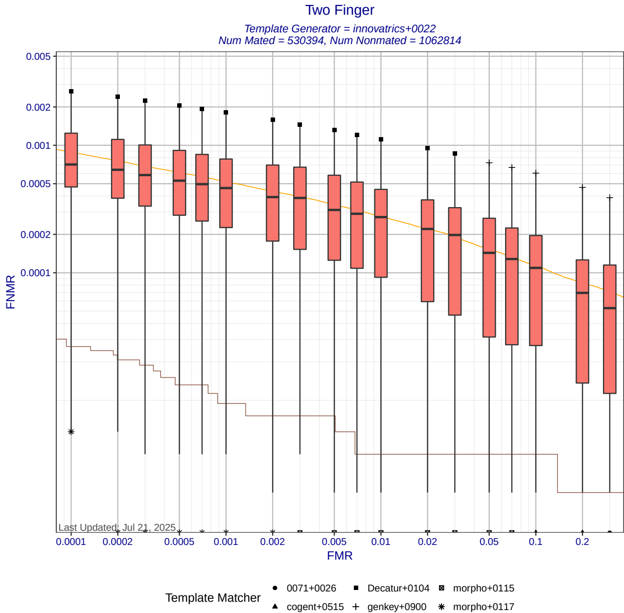
Figure 6: Two Finger DET statistics for template generator innovatrics+0022. Each box shows the distribution of FNRs at a fixed FMR across different matchers. The whisker ends show the minimum and maximum FNRs. The brown curve shows the DET curve when the matcher and template generators were submitted by the same participant. The orange DET curve shows pooled performance when all matchers use templates created by innovatrics+0022. Score-level fusion is achieved by averaging the scores for left and right index fingers.
