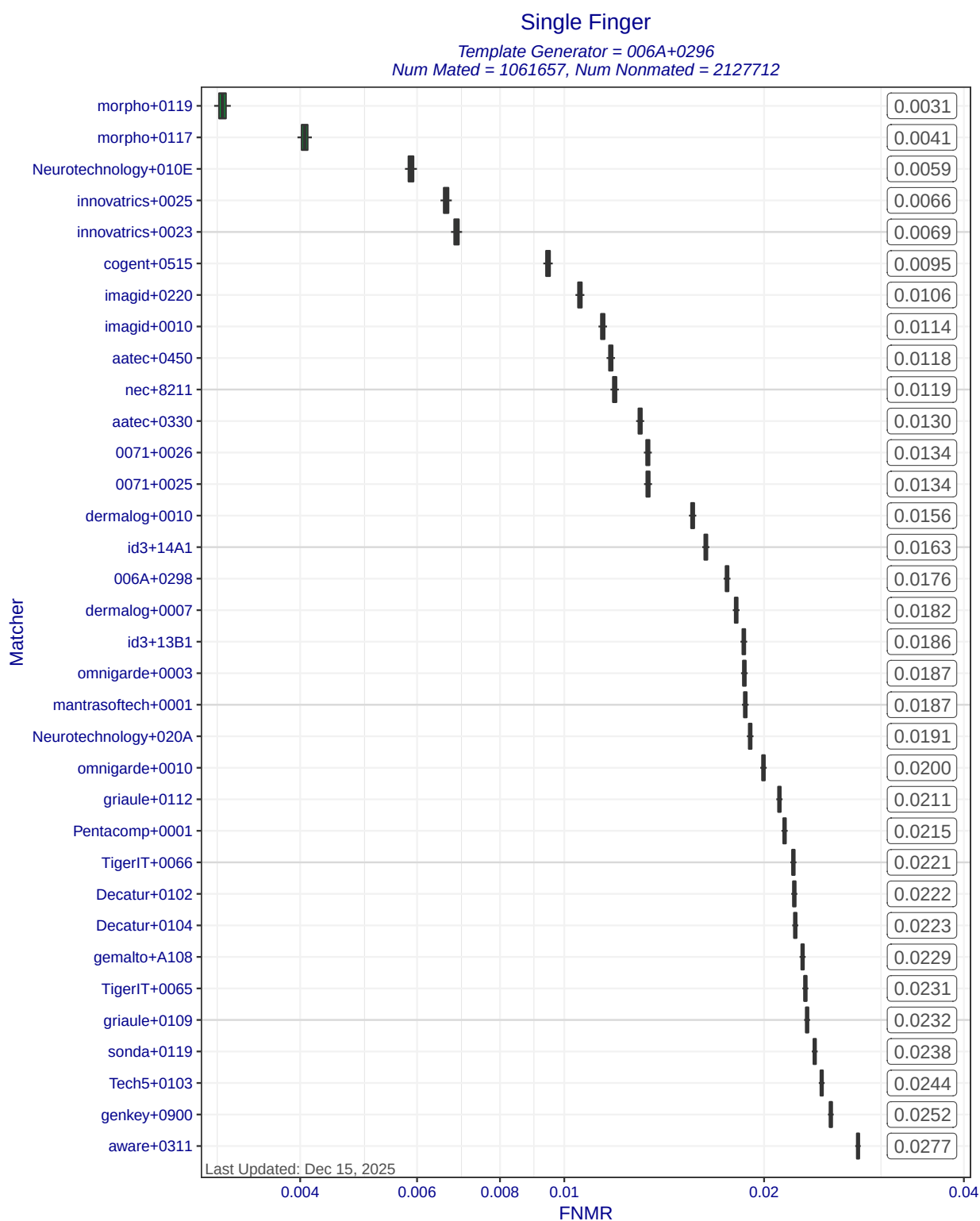
Figure 5: Single Finger FNMRs at FMR=0.0001 when MINEX III compliant matchers compare templates created by template generator 006A+0296. Each box represents uncertainty about the true FNMR. The box edges mark the 50% confidence intervals while the whiskers mark the 90% confidence intervals. The numbers on the right show the actual computed FNMRs.
