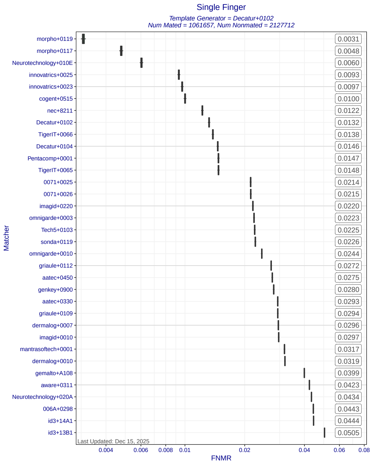
Figure 5: Single Finger FNMRs at FMR=0.0001 when MINEX III compliant matchers compare templates created by template generator Decatur+0102. Each box represents uncertainty about the true FNMR. The box edges mark the 50% confidence intervals while the whiskers mark the 90% confidence intervals. The numbers on the right show the actual computed FNMRs.
