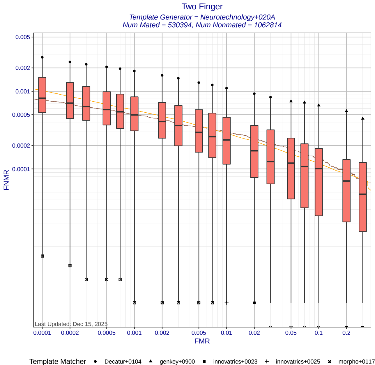
Figure 6: Two Finger DET statistics for template generator Neurotechnology+020A. Each box shows the distribution of FNMRs at a fixed FMR across different matchers. The whisker ends show the minimum and maximum FNMRs. The brown curve shows the DET curve when the matcher and template generators were submitted by the same participant. The orange DET curve shows pooled performance when all matchers use templates created by Neurotechnology+020A. Score-level fusion is achieved by averaging the scores for left and right index fingers.
