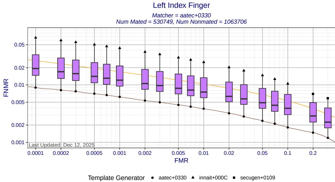
Figure 4: Left index finger DET statistics for matcher aatec+0330. Each box shows the distribution of FNRs at a fixed FMR across all MINEX III compliant template generators. The ends of the whiskers show the minimum and maximum FNRs. The orange DET curve shows pooled performance against all template generators.
