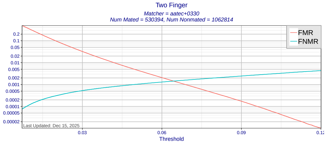
Figure 12: Two finger FMR and FNMR as a function of score threshold for matcher aatec+0330 using templates created by all MINEX III compliant template generators. Score-level fusion is achieved by averaging scores for the left and right index fingers.
