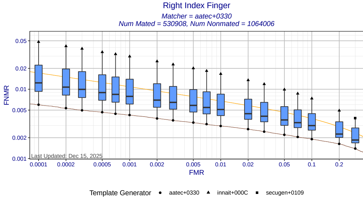
Figure 3: Right index finger DET statistics for matcher aatec+0330. Each box shows the distribution of FNR at a fixed FMR across all MINEX III compliant template generators. The ends of the whiskers show the minimum and maximum FNRs. The orange DET curve shows pooled performance against all template generators.
