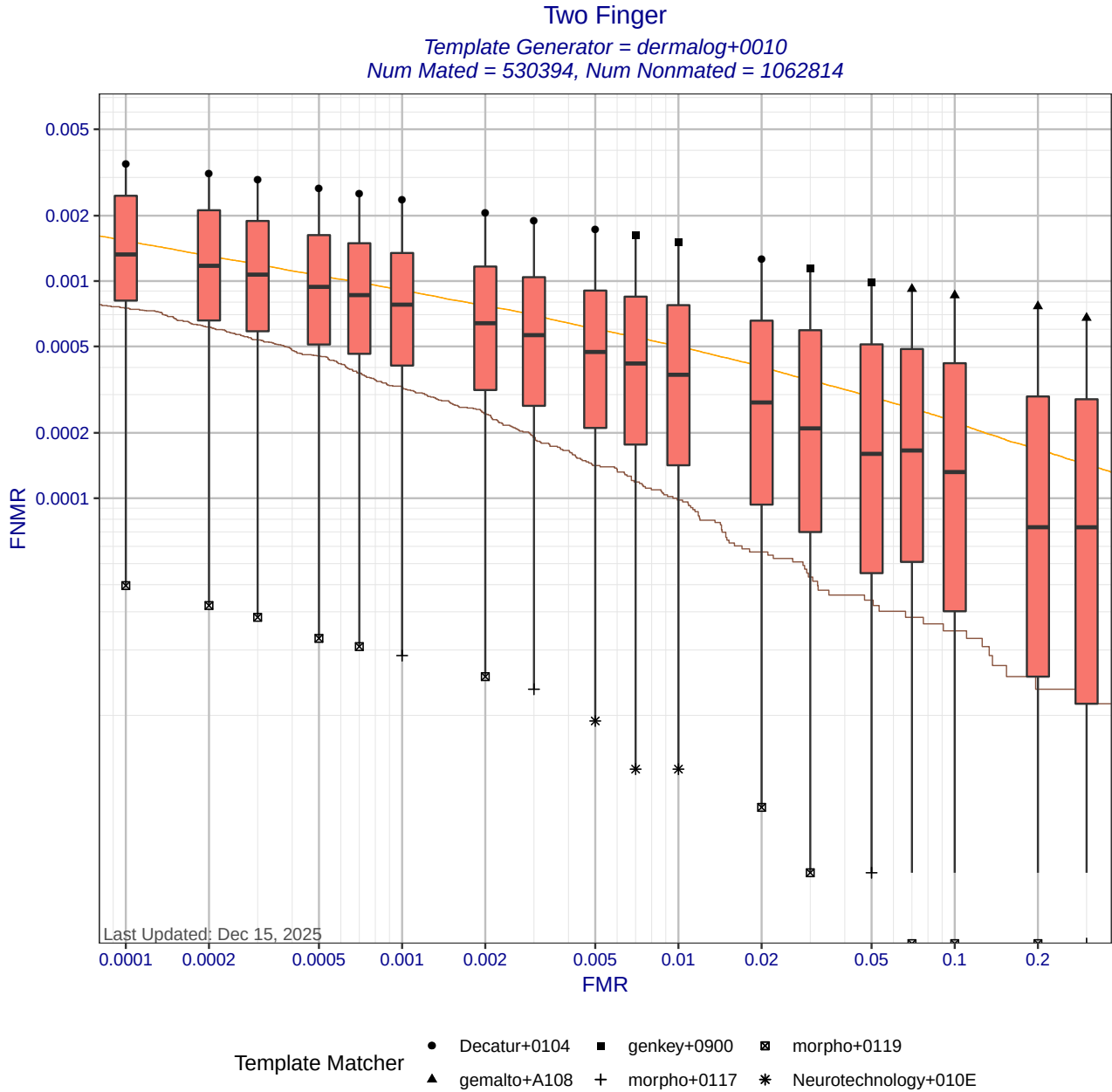
Figure 6: Two Finger DET statistics for template generator dermalog+0010. Each box shows the distribution of FNMNRs at a fixed FMR across different matchers. The whisker ends show the minimum and maximum FNMNRs. The brown curve shows the DET curve when the matcher and template generators were submitted by the same participant. The orange DET curve shows pooled performance when all matchers use templates created by dermalog+0010. Score-level fusion is achieved by averaging the scores for left and right index fingers.
