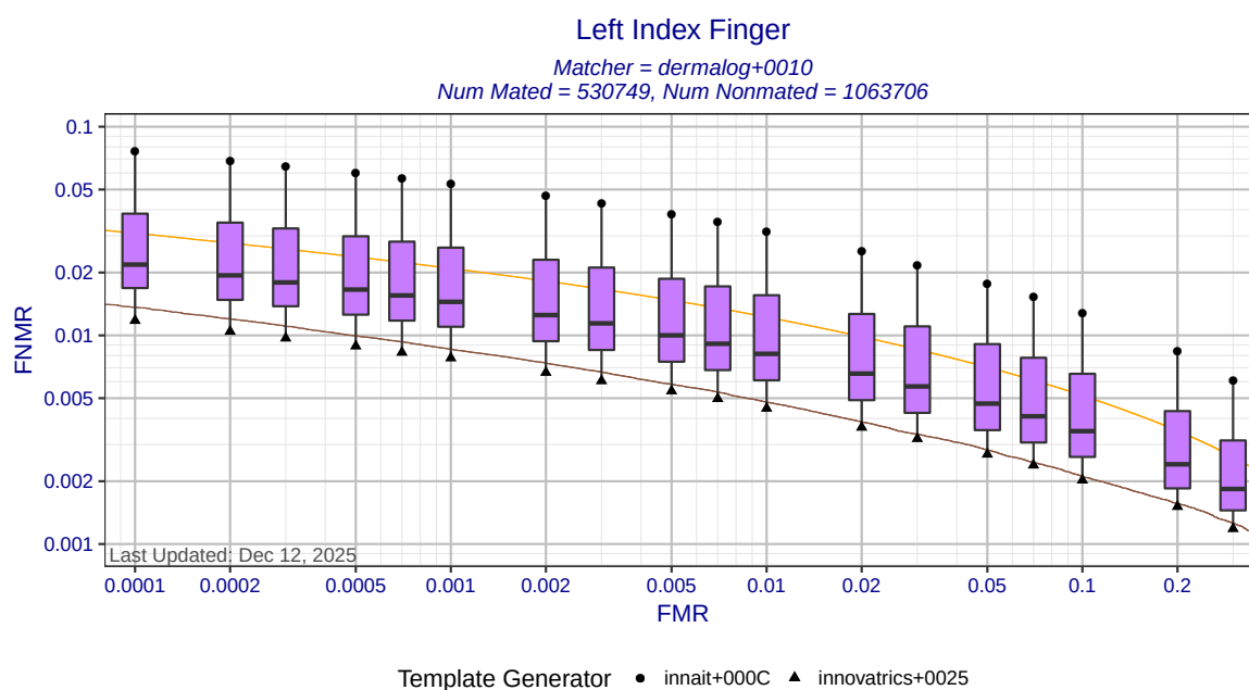
Figure 4: Left index finger DET statistics for matcher dermalog+0010. Each box shows the distribution of FNMRs at a fixed FMR across all MINEX III compliant template generators. The ends of the whiskers show the minimum and maximum FNMRs. The orange DET curve shows pooled performance against all template generators.
