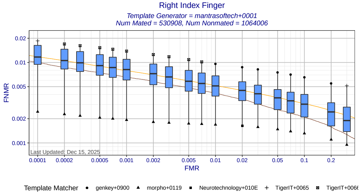
Figure 3: Right Index Finger DET statistics for template generator mantrasoftech+0001. Each box shows the distribution of FNMRs at a fixed FMR across different matchers. The whisker ends show the minimum and maximum FNMRs. The brown curve shows the DET curve when the matcher and template generators were submitted by the same participant. The orange DET curve shows pooled performance when all matchers use templates created by mantrasoftech+0001.
