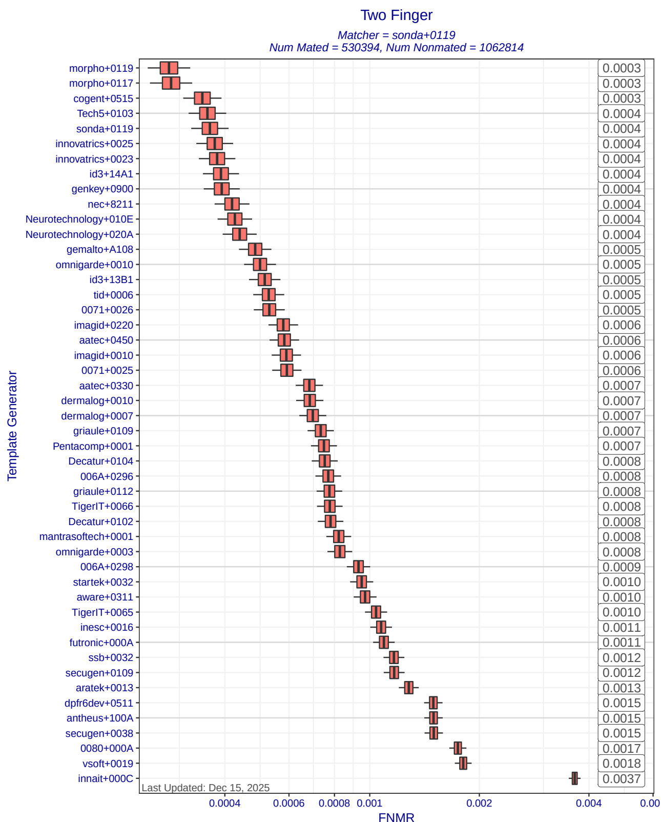
Figure 8: Two finger FNMR at FMR=0.01 when matcher sonda+0119 compares templates created by different template generators. Each box represents uncertainty about the true FNMR. The box edges mark the 50% confidence intervals while the whiskers mark the 90% confidence intervals. The numbers on the right show the actual computed FNMRs. Score-level fusion is achieved by averaging the scores for left and right index fingers.
