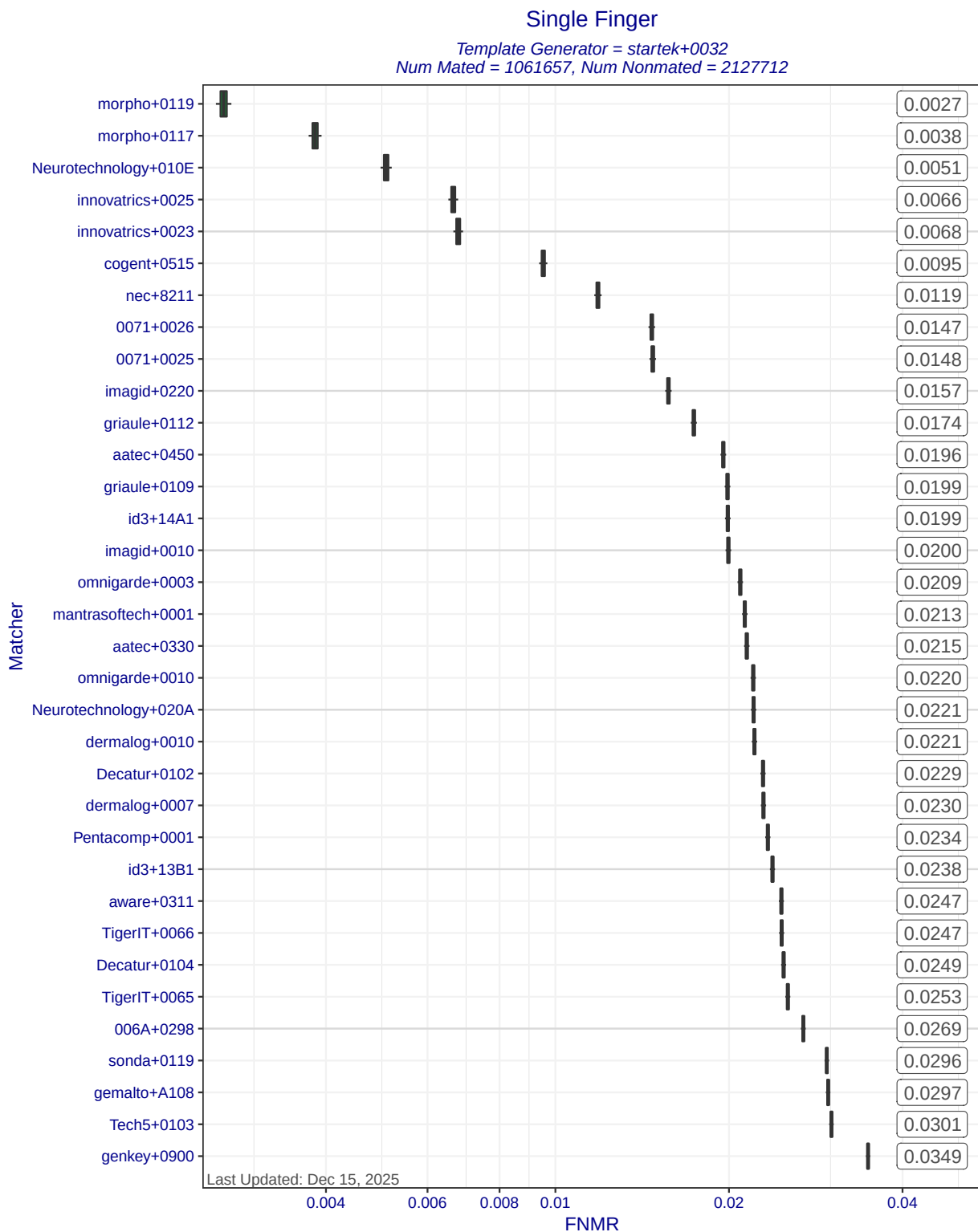
Figure 5: Single Finger FNMRS at FMR=0.0001 when MINEX III compliant matchers compare templates created by template generator startek+0032. Each box represents uncertainty about the true FNMRS. The box edges mark the 50% confidence intervals while the whiskers mark the 90% confidence intervals. The numbers on the right show the actual computed FNMRS.
