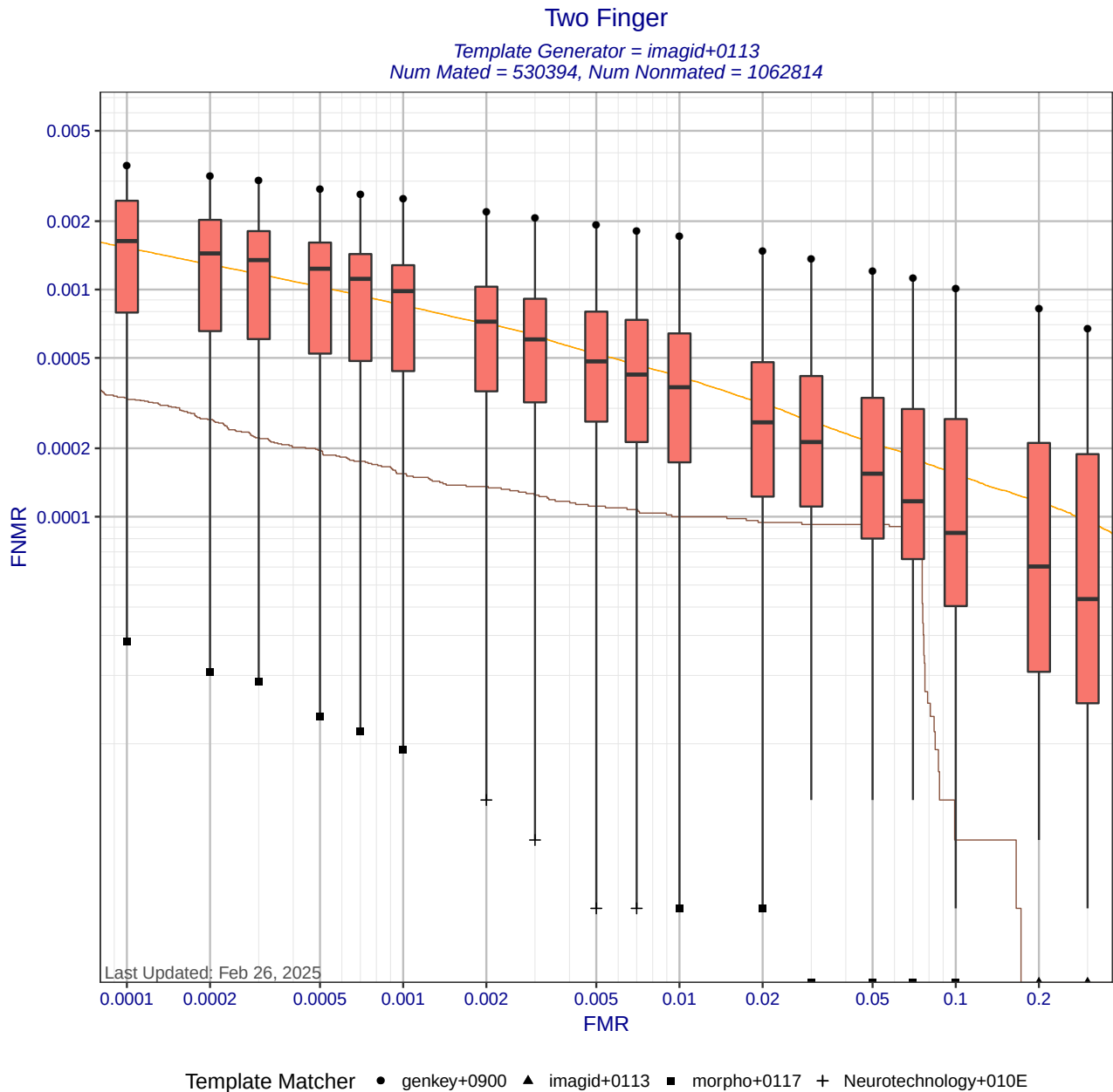
Figure 6: Two Finger DET statistics for template generator imagid+0113. Each box shows the distribution of FNMIRs at a fixed FMR across different matchers. The whisker ends show the minimum and maximum FNMIRs. The brown curve shows the DET curve when the matcher and template generators were submitted by the same participant. The orange DET curve shows pooled performance when all matchers use templates created by imagid+0113. Score-level fusion is achieved by averaging the scores for left and right index fingers.
