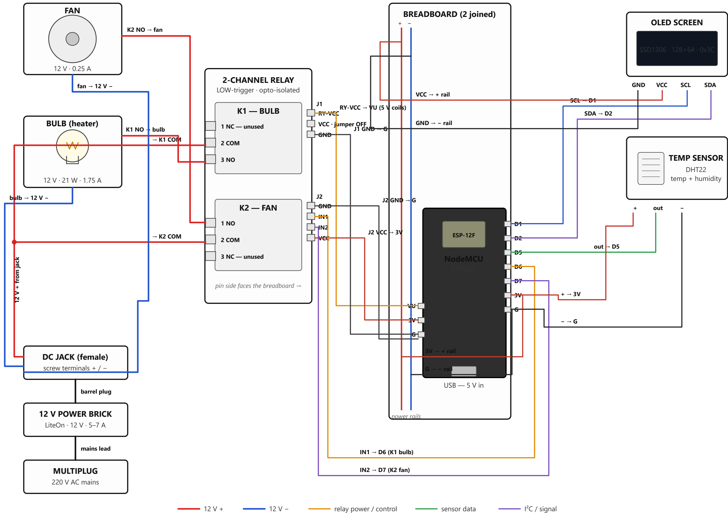
microaqila — circuit diagram (as built) Layout matches the bench photo · NodeMCU ESP8266 · DHT22 · SSD1306 OLED · 2-channel relay · 12 V fan + 12 V bulb
