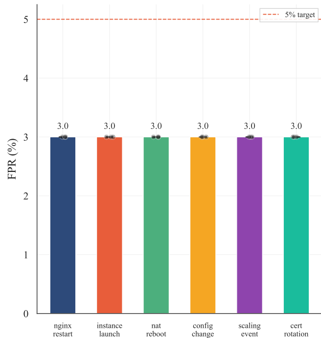
(a) Post-Drift False Positive Rate
