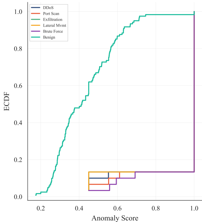
(b) Score ECDF by Context
