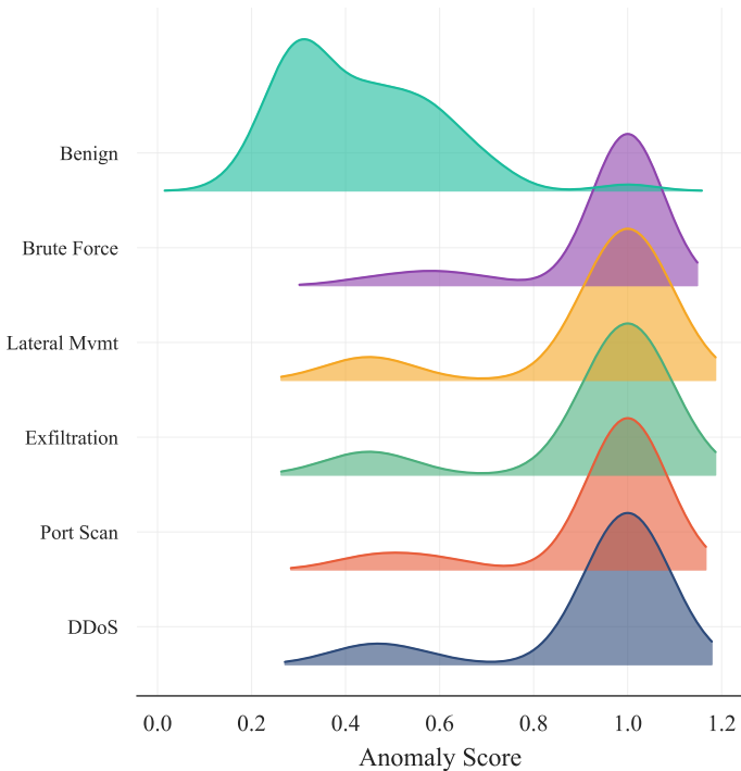
(a) Score Distribution by Context
