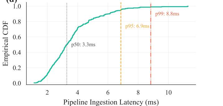
(c) Network Packet Rate Distribution — simulated (no AWS capture available) (d) Pipeline Ingestion Latency ECDF — simulated (no AWS capture available)
