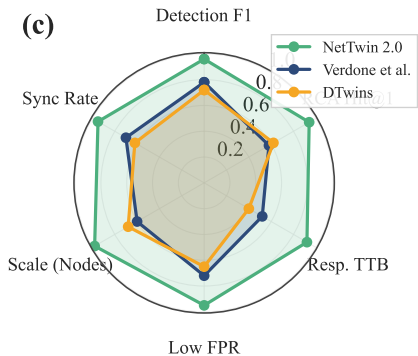
(c) Multi-Dimensional Performance Radar
