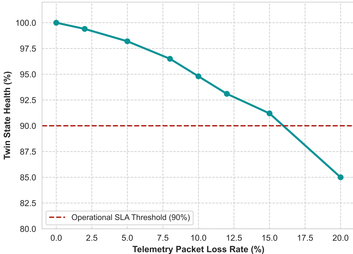
(a) Digital Twin Health under Packet Loss
