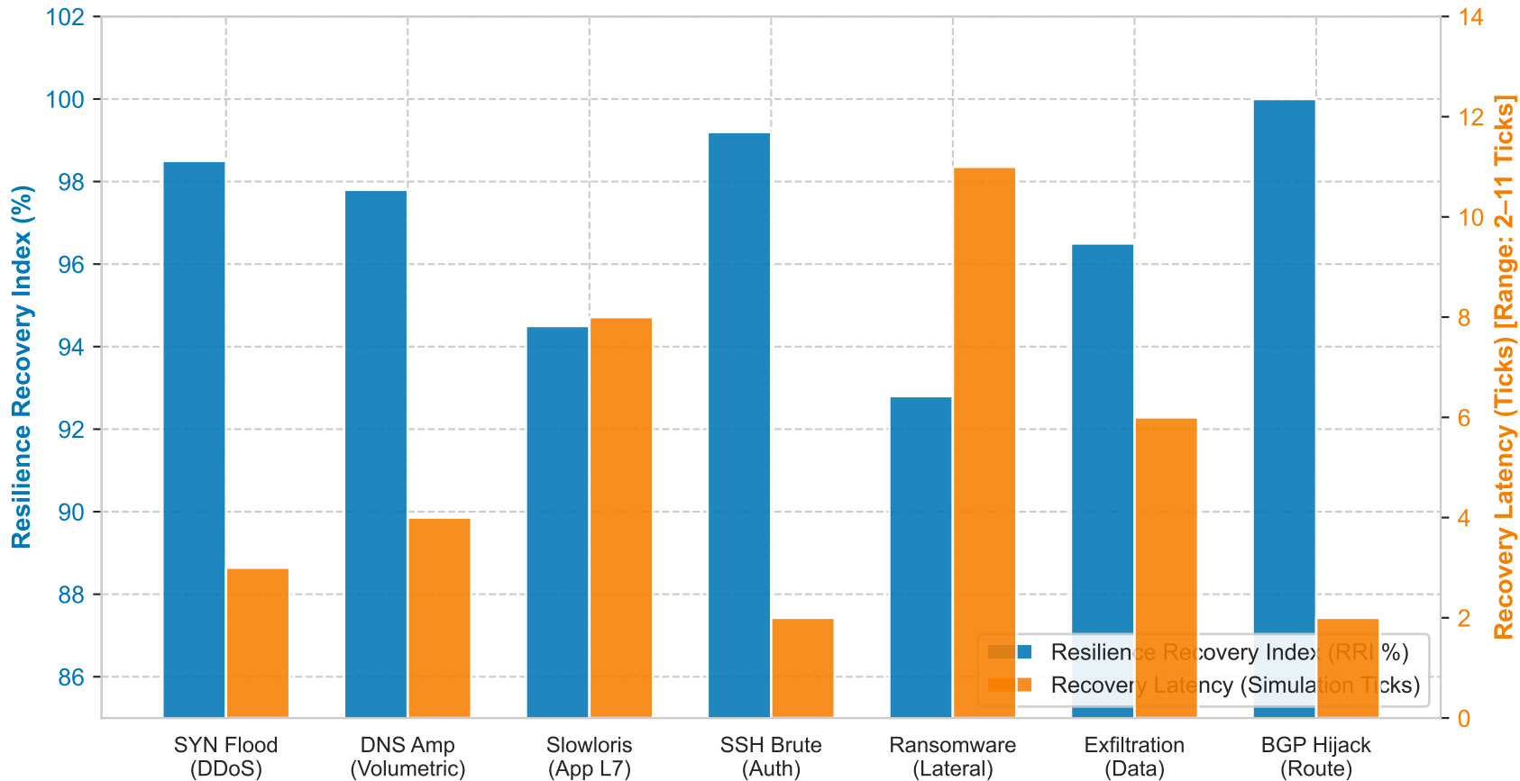
Paper 4 [ACM CCS] — Table B: Multi-Threat Resilience Profile Rapid Autonomous Containment Across 7 Distinct Attack Scenarios (RRI \geq 0.928 )
