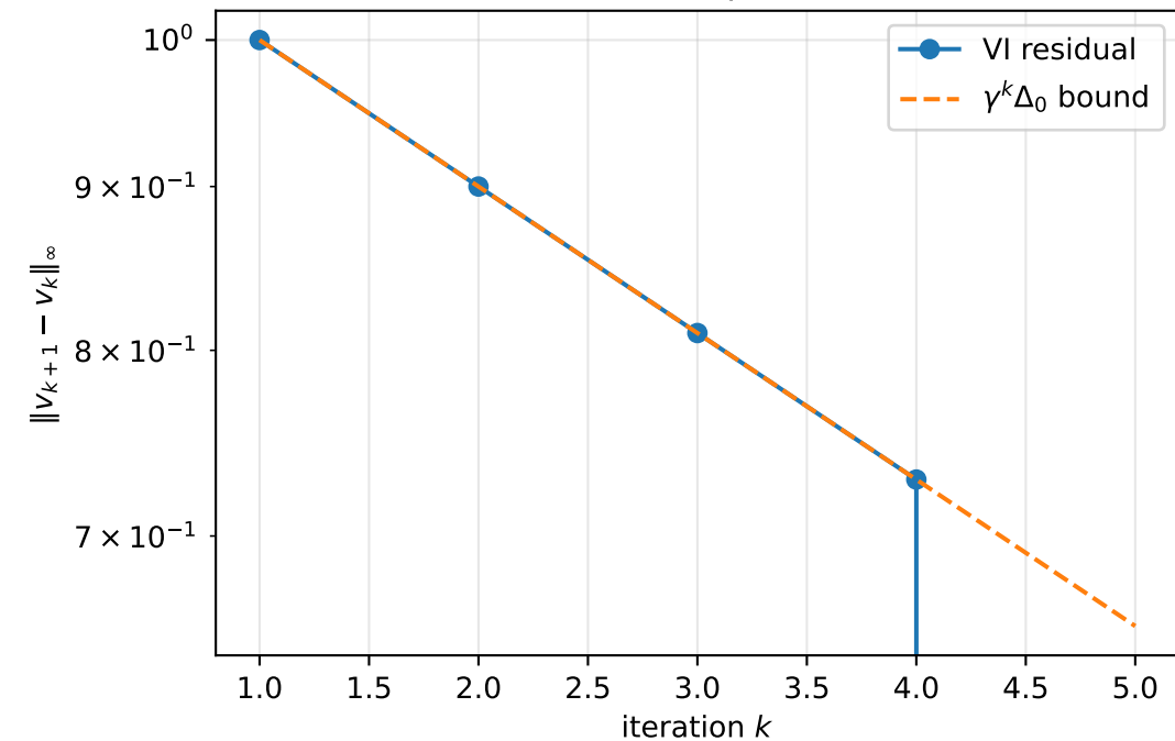
Value Iteration: \gamma -contraction
