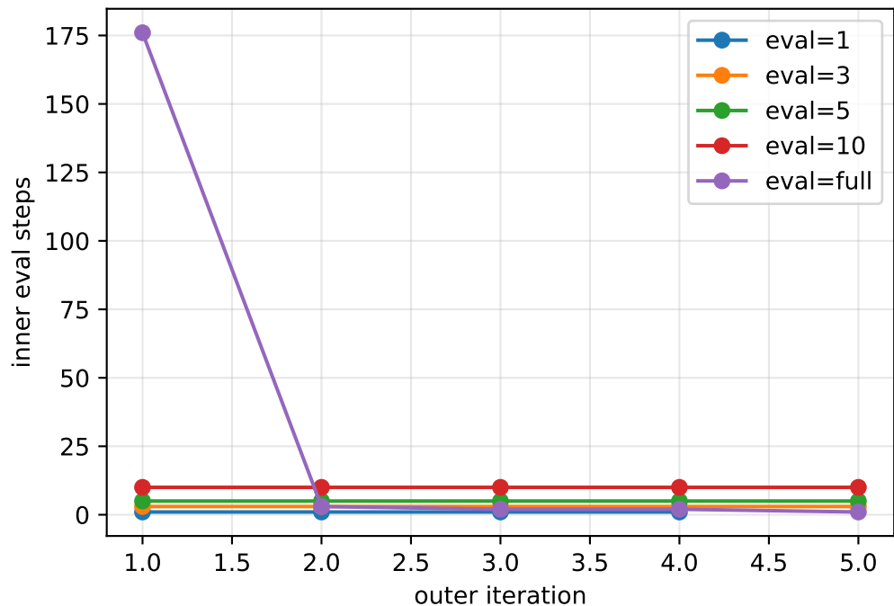
Truncated PI vs Full PI
