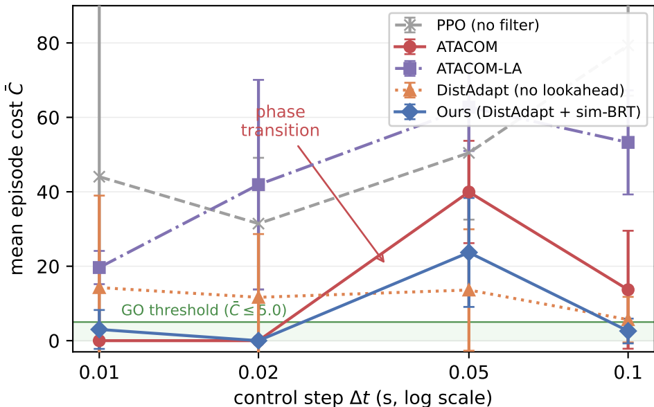
Filter-zoo phase transition at \Delta t \approx 0.05 s
