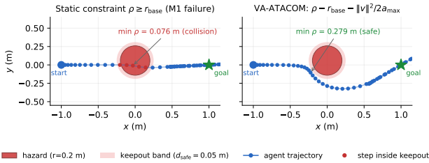
Figure 1: Why velocity augmentation matters (double-integrator, \Delta t=0.1 s, v_{\text{max}}=1 , a_{\text{max}}=0.9 ). Same tangent projection in both panels; only the constraint differs. Left , static \rho \geq r_{\text{base}} : momentum carries the agent through to \rho_{\text{min}}=0.076 m (collision, M1/M2). Right , VA-ATACOM: the braking term decelerates early, \rho_{\text{min}}=0.28 m (Table 2).
