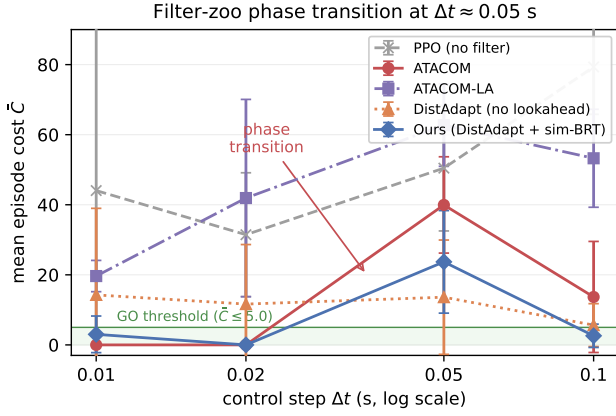
Figure 3: Filter-zoo phase transition at \Delta t \approx 0.05 s. Mean episode cost \bar{C} versus control step \Delta t on SafetyPointGoal1-v0 (5 filters \times 4 \Delta t values \times 3 seeds \times 50K env steps). Vertical bars show \pm 1 standard deviation across seeds. The green band is the GO threshold ( \bar{C} \leq 5 , the convention used throughout §III-A). Red , ATACOM: zero cost at \Delta t \leq 0.02 s (the regime where the continuous-time forward-invariance theorem of §III-B holds empirically) and catastrophic at \Delta t \geq 0.05 s — a clean phase transition consistent with the M1 threshold (Prop. 1, §IV-A). Purple , ATACOM-LA: uniformly poor across \Delta t — the 1-step lookahead does not save the family and introduces over- conservatism artefacts (§VI-A). Orange , DistAdapt (no lookahead) and grey , PPO baseline: the velocity-margin alone is insufficient; the no-filter baseline is uniformly catastrophic. Blue , Ours (DistAdapt + sim-BRT): stays in the GO band at every \Delta t except the corner cell at \Delta t = 0.05 s where h \cdot \Delta t = 0.15 s straddles the M2 drift timescale (discussed in §VI-C).
