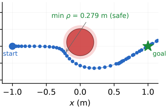
VA-ATACOM: \rho - r_{\text{base}} - \|v\|^2/2a_{\text{max}}
