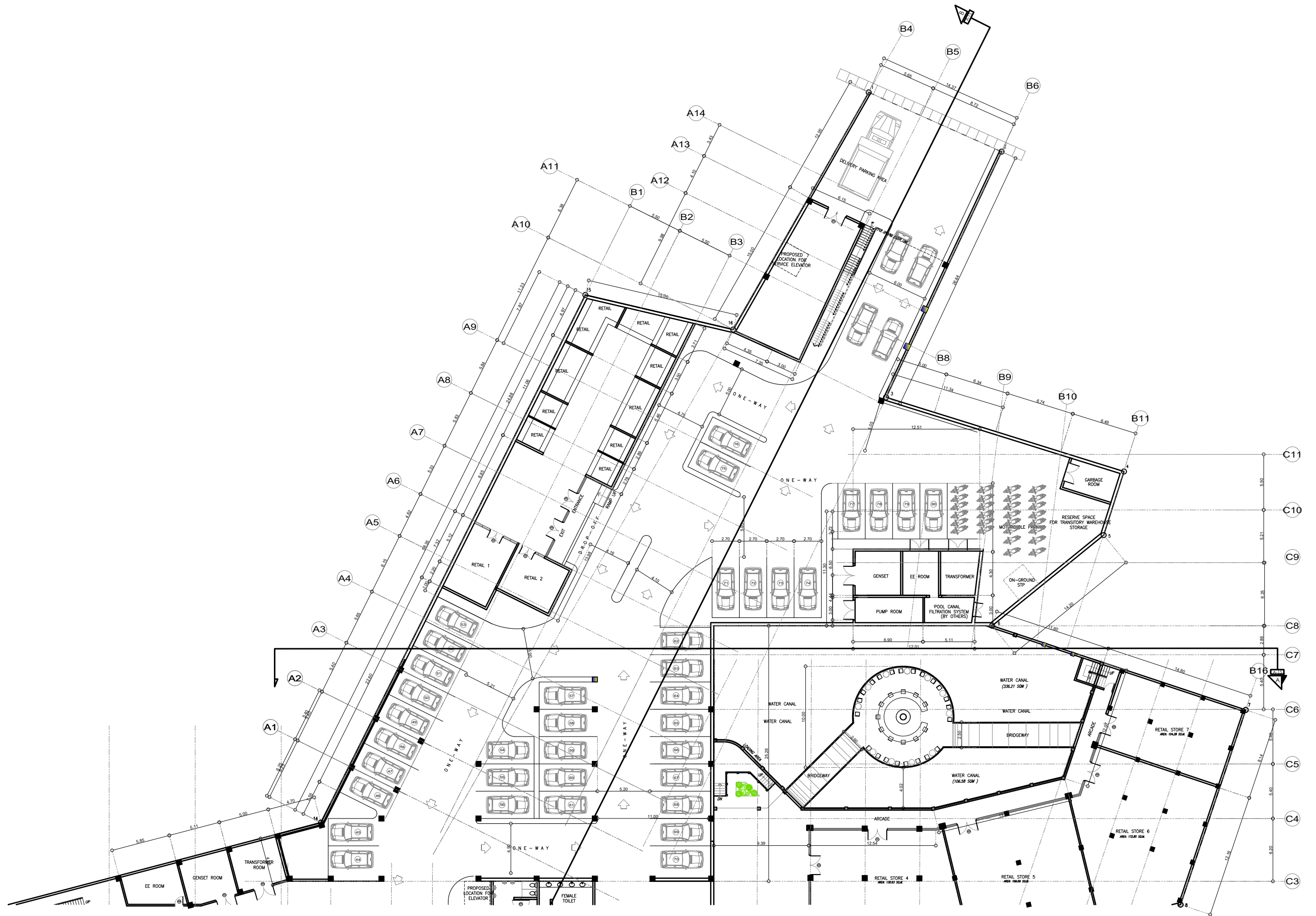
LOWER PORTION LOWER GROUND FLOOR PLAN SCALE: 1:100 N.E.
