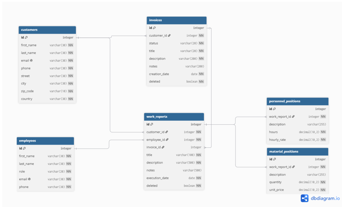
Figure 7: Entity-Relation diagram
