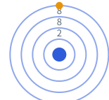
K (2, 8, 8, 1)
