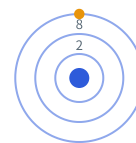
Na (2, 8, 1)
