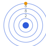
K (2, 8, 8, 1)
