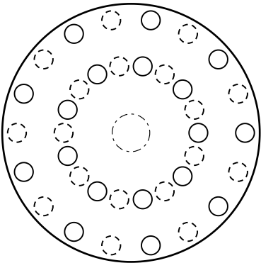
CLOSED POSITION – TOP PLATE +20.0° (DASHED) EVERY HOLE ON SOLID WEB, .441 MIN COVER
