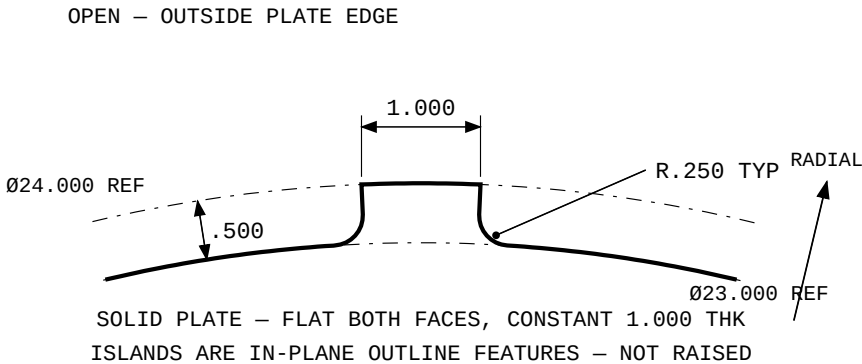
4) DETAIL B – PLAN, TRUE CURVATURE
