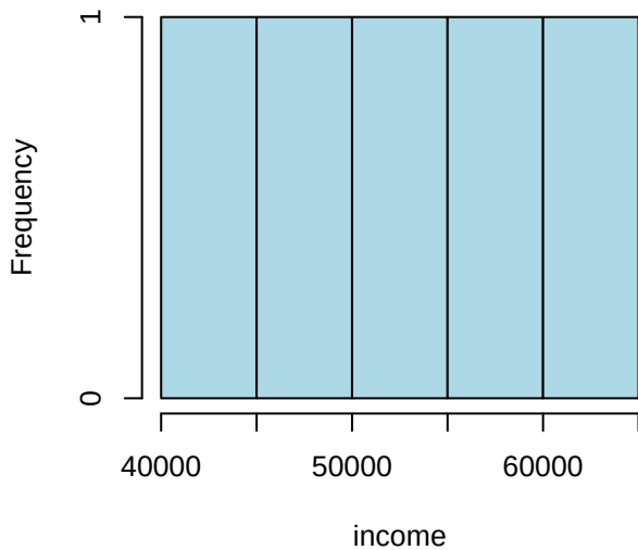
Histogram of income
