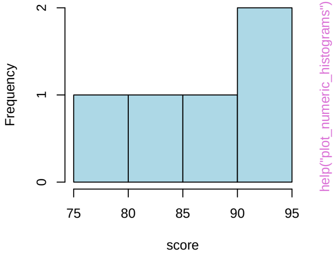
Histogram of score
