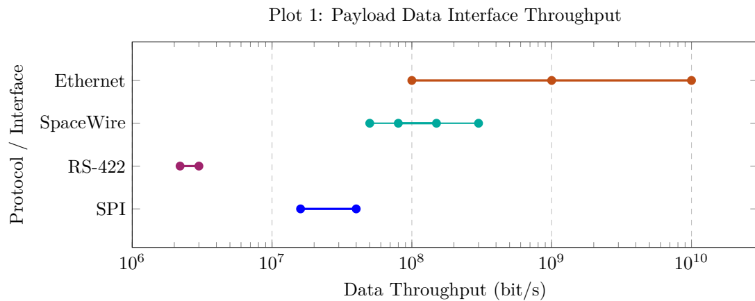
Figure 2: Published payload data interface rates from the commercial OBC survey (Appendix B). Values may be measured, manufacturer-stated, or nominal depending on the source; dots represent specific published figures and lines represent observed ranges. Practical application-level throughput is considered separately in Table 7.
