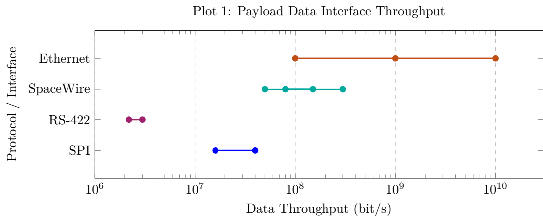
Figure 2: Observed payload data interface throughputs from commercial OBC survey (Appendix B). Dots represent specific published figures; lines represent observed operational ranges.
