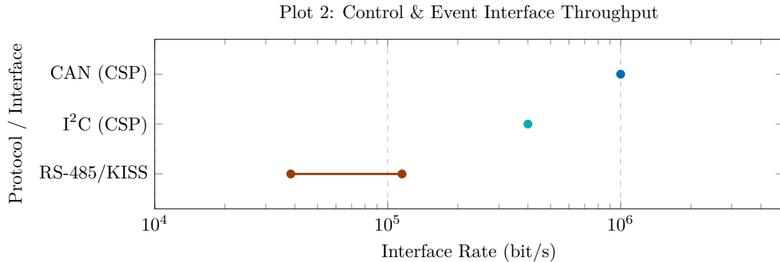
Figure 3: Observed control throughput and event interface rates from commercial OBC survey (Appendix B).
