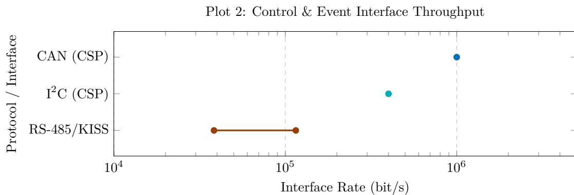
Figure 2: Published control and event interface rates from the commercial OBC survey (Appendix B). These values are configured or published interface rates and should not be interpreted directly as application goodput; see Table 7.
