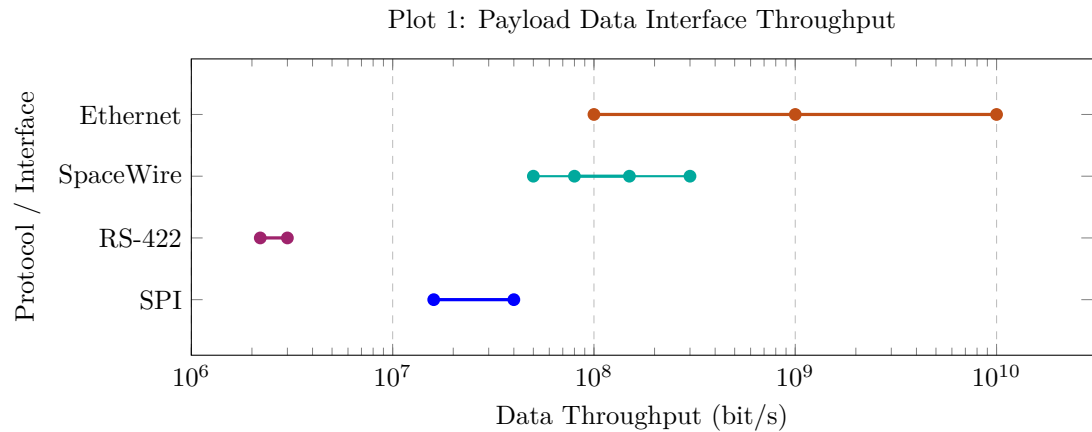
Figure 1: Published payload data interface rates from the commercial OBC survey (Appendix B). Values may be measured, manufacturer-stated, or nominal depending on the source; dots represent specific published figures and lines represent observed ranges. Practical application-level throughput is considered separately in Table 7.
