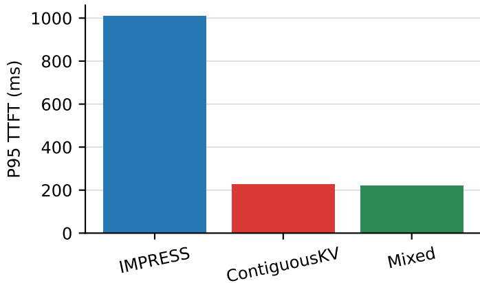
SST-2
