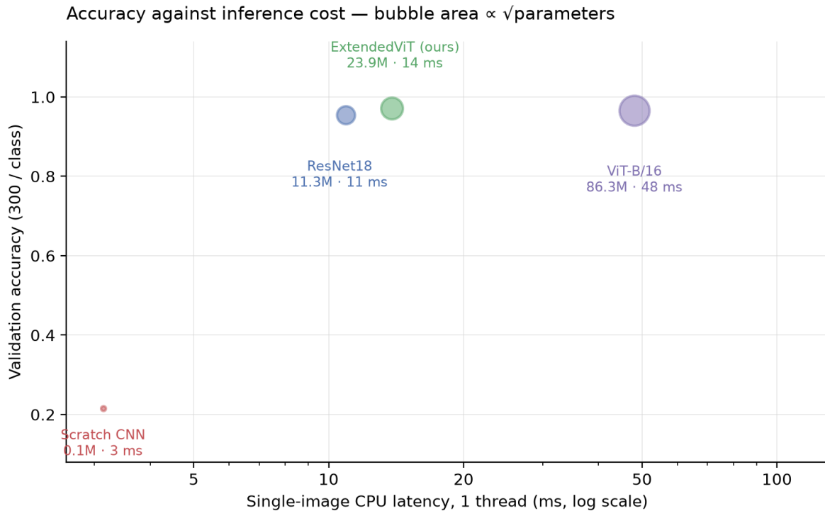
Figure 9. Accuracy against single-image CPU latency; bubble area is proportional to the square root of parameter count.
