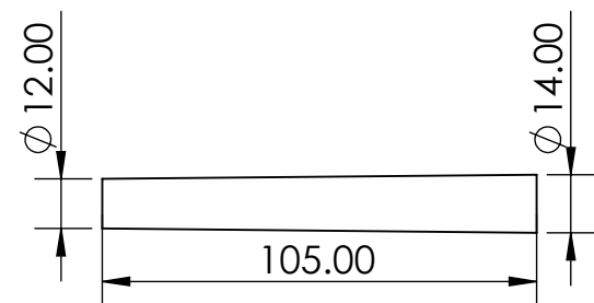
Figure 12 Pivot Pin
