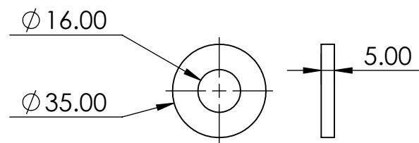
Figure 4 Small Washer
