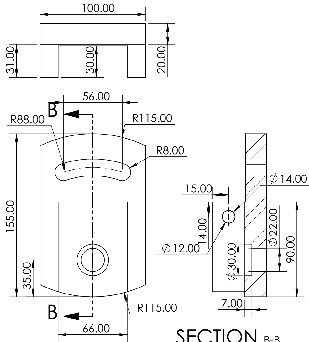
Figure 2 Swivel Plate
