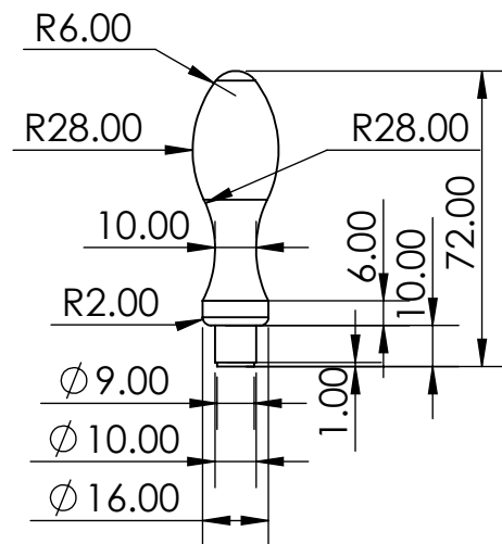
Figure 9 Handle
