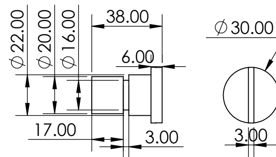
Figure 10 Swivel Screw Pin
