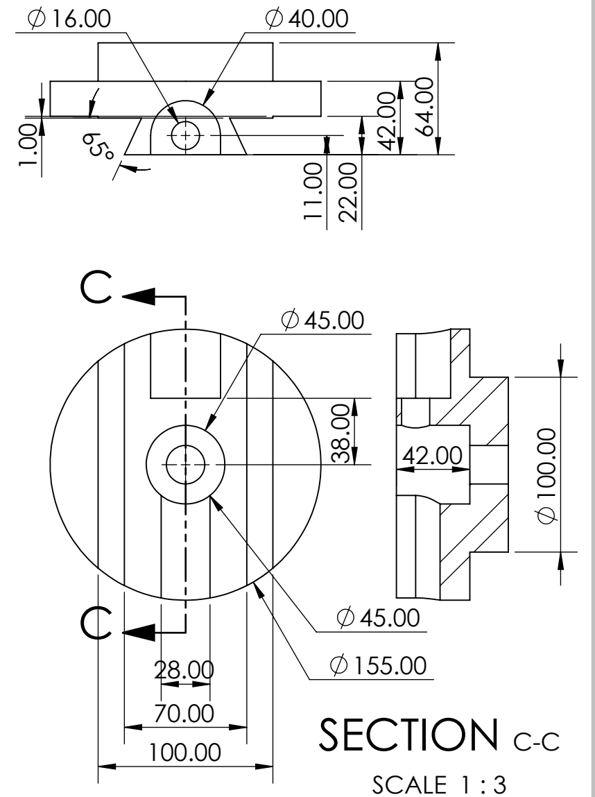
Figure 5 Back Plate
