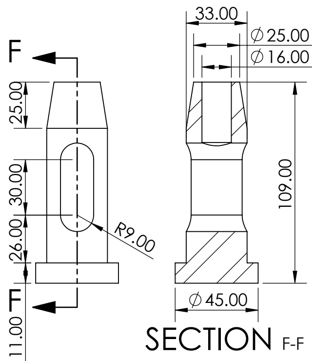
Figure 14 Tool Holder
