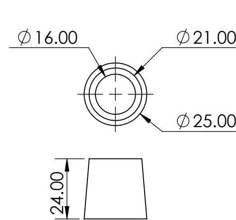
Figure 7 Spacer Bush
