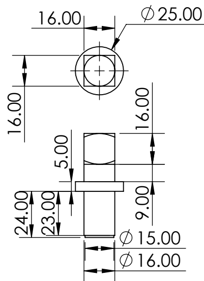
Figure 3 Clamping View
