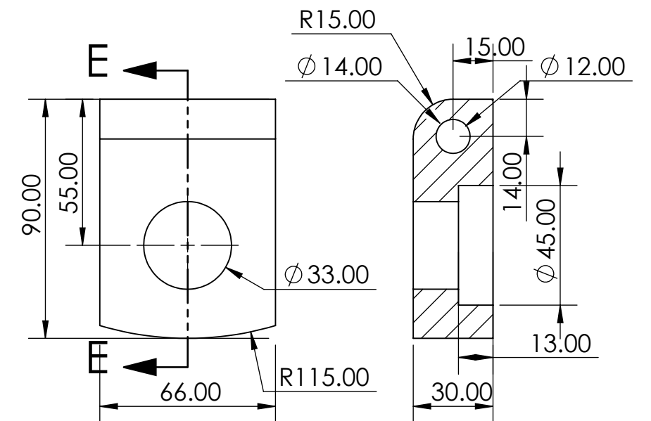
SECTION E-E
