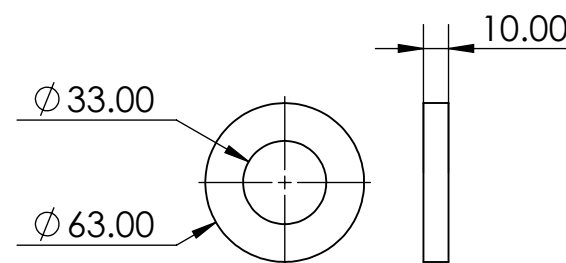
Figure 15 Washer
