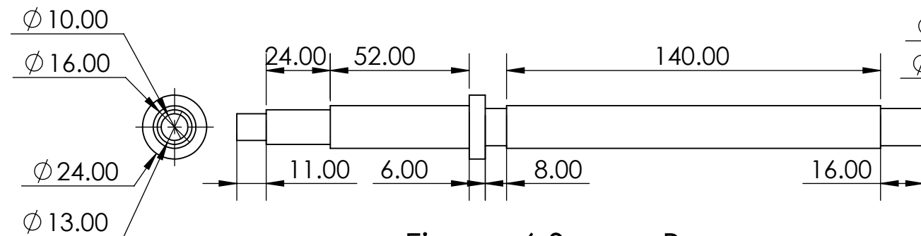
Figure 6 Screw Bar
