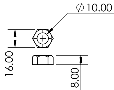
Figure 16 Nut
