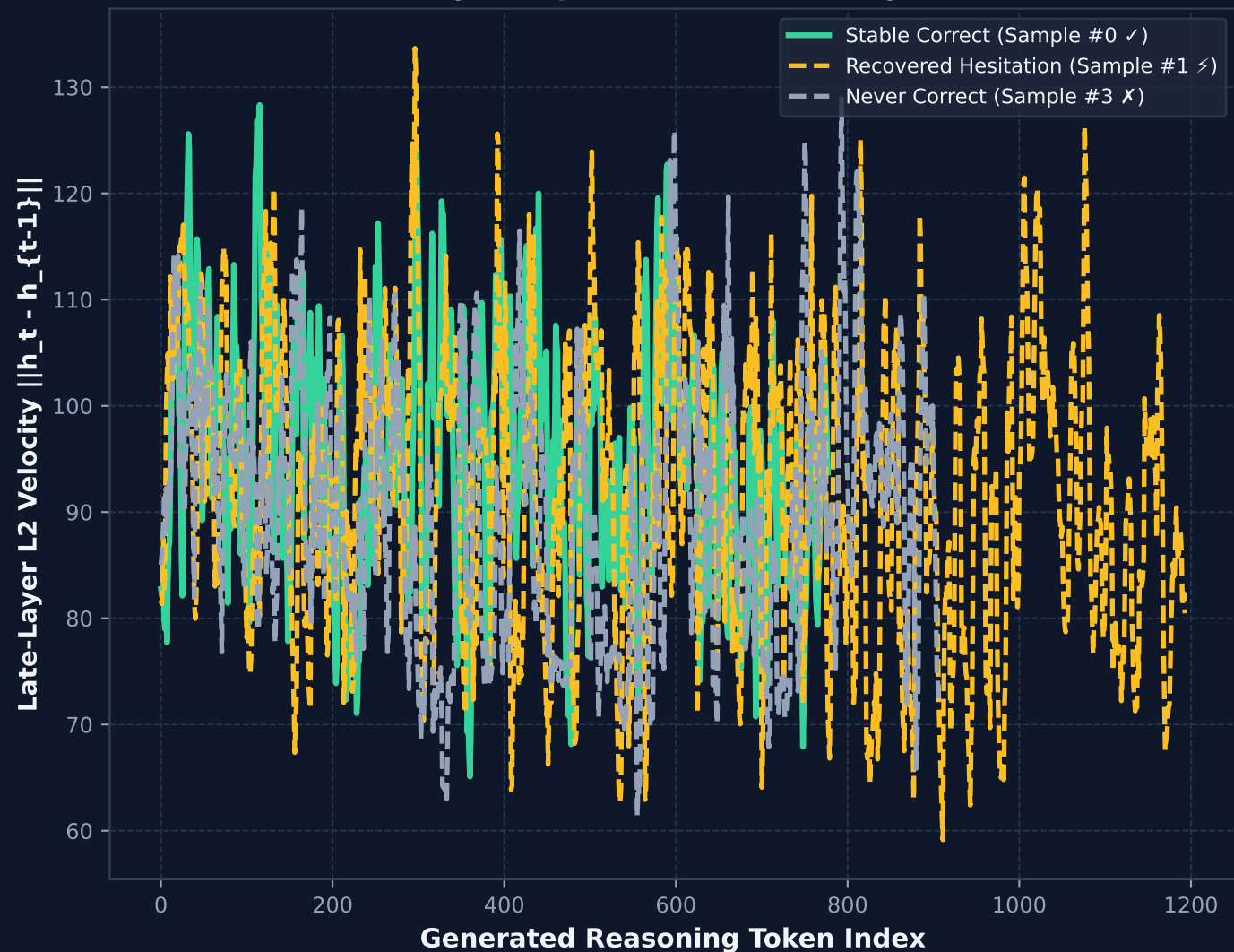
Panel A: Real Late-Layer Representation Velocity (L2 Movement)
