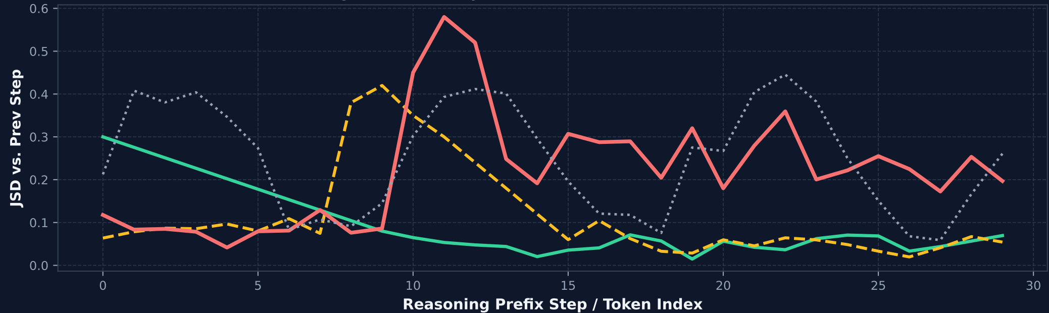
Panel C: Jensen-Shannon Divergence Volatility (Distributional Shock)
