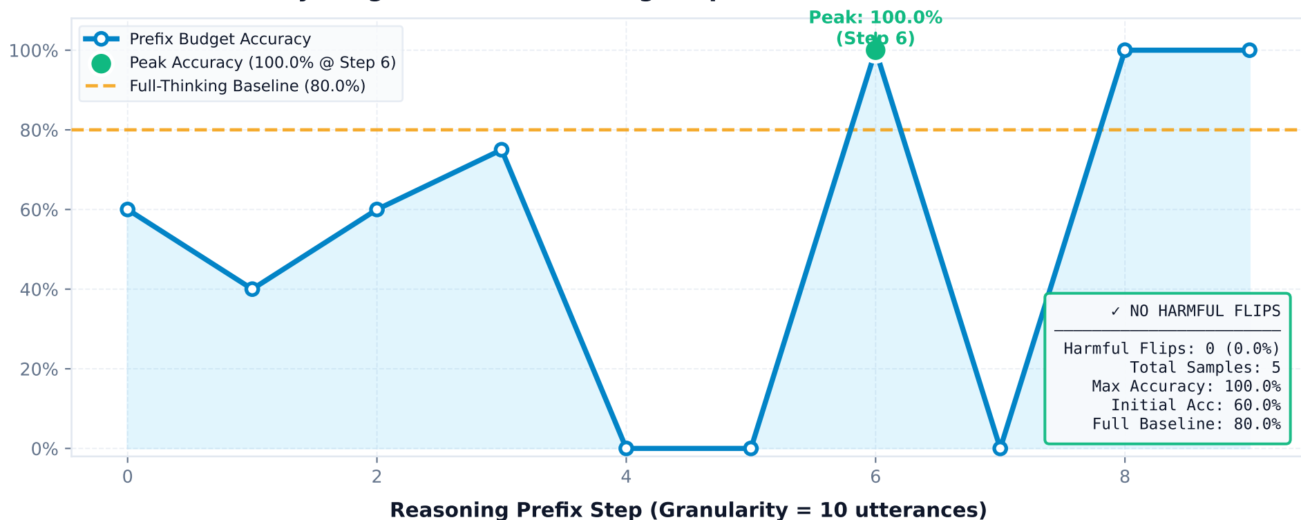
Panel A: Accuracy Progression vs. Thinking Step
