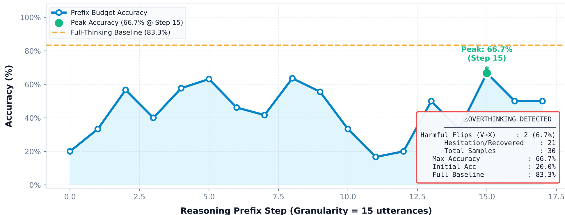
Panel A: Accuracy Progression vs. Thinking Step (r1_distill_qwen1_5b on gsm8k)
