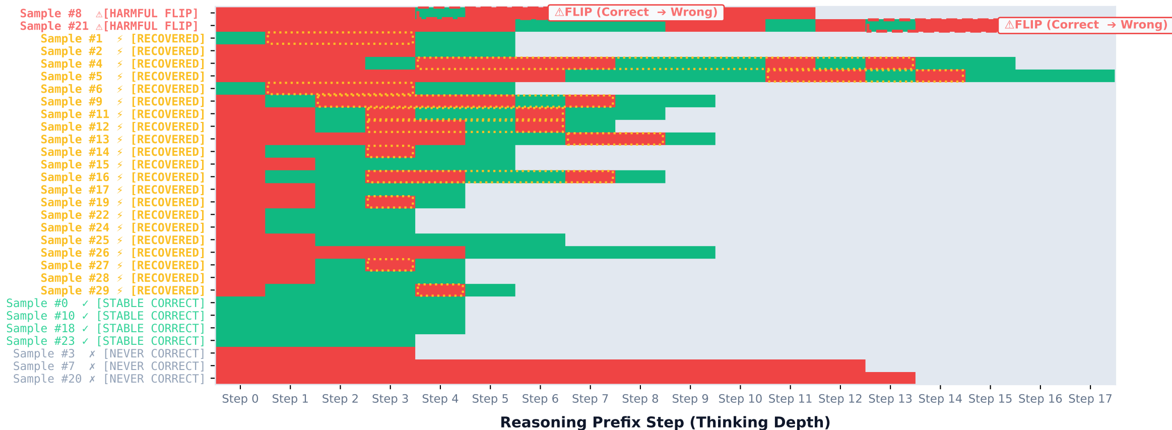
Panel B: Reasoning Trajectories by Archetype (✖ Correct | ✖ Incorrect | ✎ Completed)
